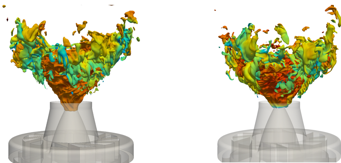
Static mesh: 877 M elements / \Delta_{FF} = 150 \mu m Adapted mesh: 260 M elements / \Delta_{FF} = 150 \mu m Figure 2: Iso-contour of the progress variable @ 0,7, colored with the temperature field. Simulation of the PRECCINSTA burner presented at the ICNC conference [5].
