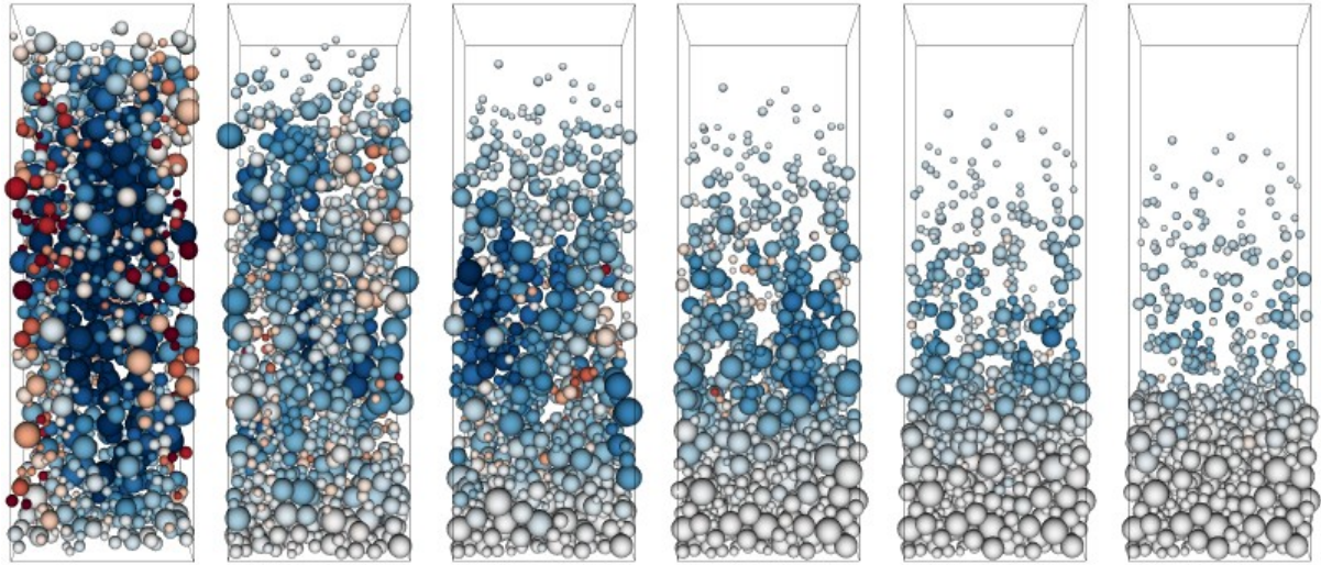
Grain-resolving DNS simulations of cohesive sediment.
